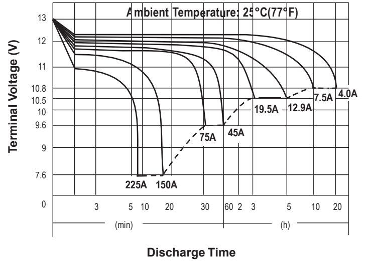
Discharge Characteristics
